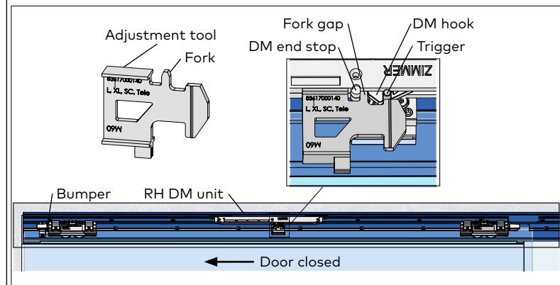
Fig. 16.5 DM unit end stop and hook separation adjustment Adjustment tool Fork Fork gap DM end stop DM hook Trigger
