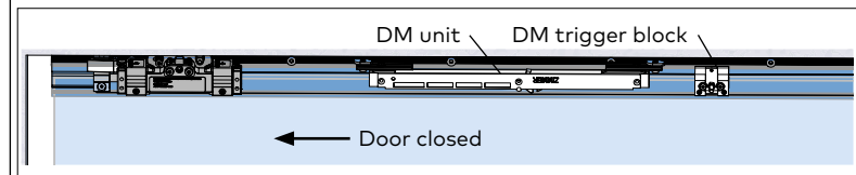
Fig. 16.3 RH DM unit inserted in track
