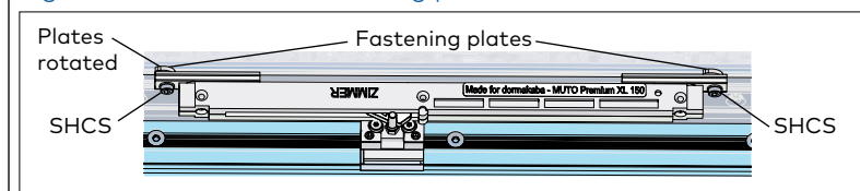
Fig. 16.14 LH DM unit fastening plates secured in track
