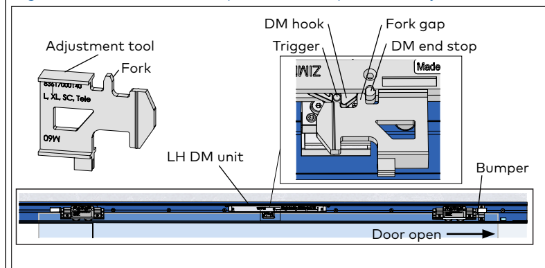
Fig. 16.13 DM unit end stop and hook separation adjustment
