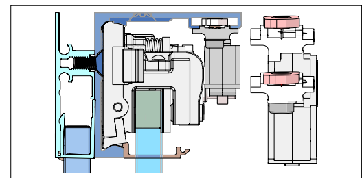
Fig. 16.7 RH DM unit aligned in track
