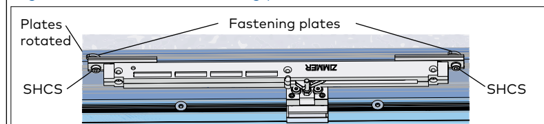
Fig. 16.6 RH DM unit fastening plates secured in track Plates rotated Fastening plates SHCS
