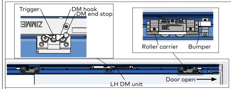
Fig. 16.12 DM unit hook positioned in trigger
