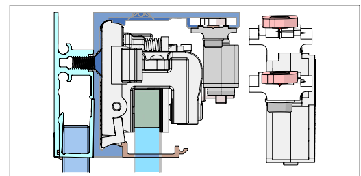
Fig. 16.15 LH DM unit aligned in track
