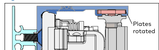
Fig. 16.8 RH DM unit installed in track
