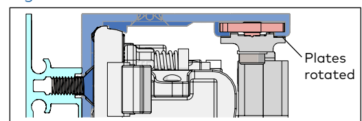
Fig. 16.16 LH DM unit installed in track
